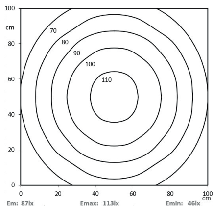
HELULIGHT® CLASSIC 140 mm (11024032, 11024038)
