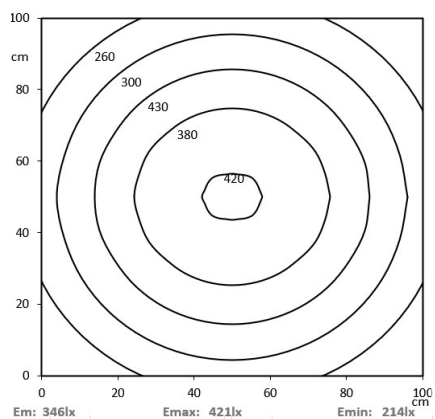
HELULIGHT® CLASSIC 560 mm (11023408, 11024041)
