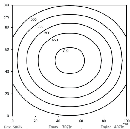
HELULIGHT® CLASSIC 980 mm (11024036, 11029460)
