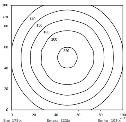
HELULIGHT® CLASSIC 280 mm (11023407, 11024039)
