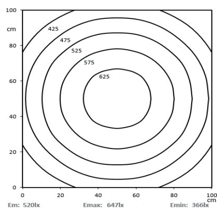
HELULIGHT® CLASSIC 840 mm (11024035, 11024043)
