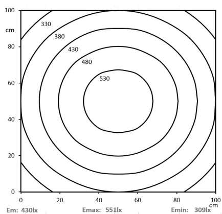
HELULIGHT® CLASSIC 700 mm (11024034, 11024042)
