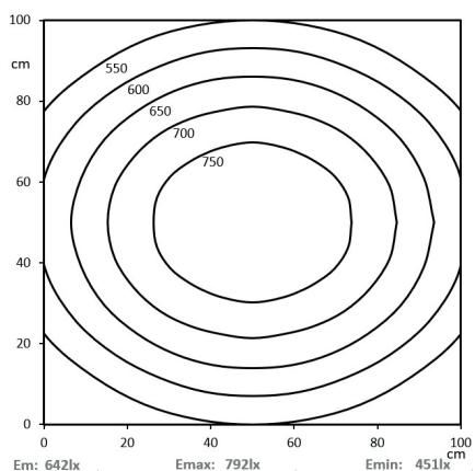
HELULIGHT® CLASSIC 1120 mm (11023409, 11029462)
